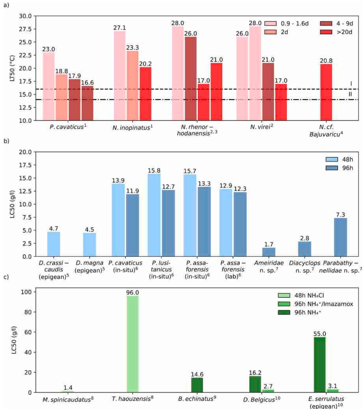
Fig. 3. Results from dose-response tests for a) temperature sensitivity of stygobiontic species, I – threshold estimated by Briellmann et al. (2011), II – threshold estimated by Spengler (2017); b) lethal concentration of 50% of the tested individuals (LC50) for NaCl; c) lethal concentrations of 50% of the tested individuals (LC50) for ammonium species and mixtures.
