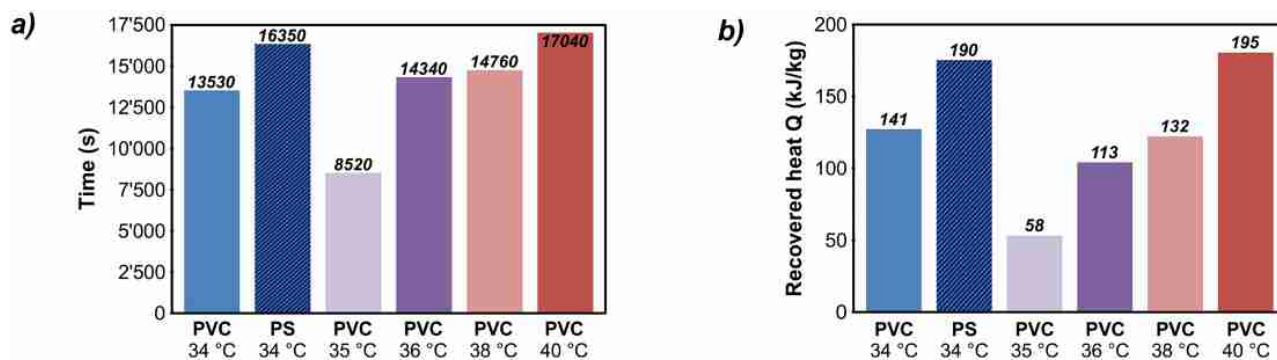
Fig 8. a) Delay in cooling of laboratory heat storage due to paraffin wax solidification; b) additional released heat by paraffin wax measured in the cooling phase. PVC: polyvinylchloride, PS: polystyrene glass plates.
