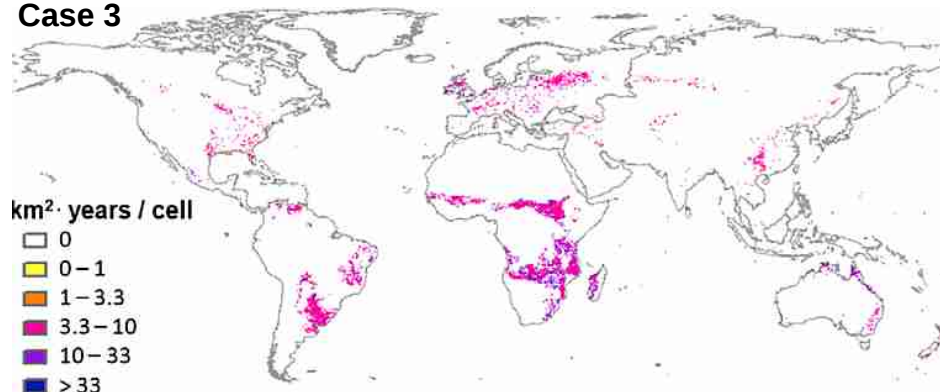
Fig. 5. Increased annual land stress due to expansion measured as \text{km}^2 \cdot \text{year} per grid cell (5 arc-minute grid): exclusive expansion on pastures in Cases 2 and 4 (top) and on pastures and natural ecosystems in Case 3 (bottom).
